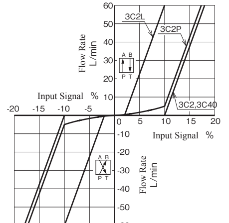
Around Null Position Input Signal -20↔+20%
